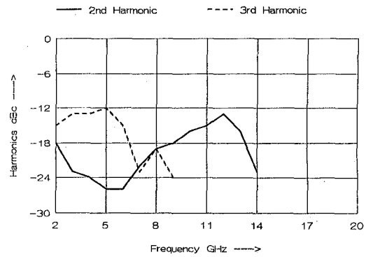
Fig.5 Inband 2nd & 3rd Harmonic
