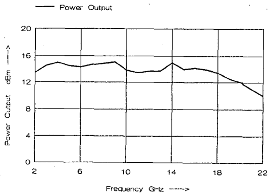
Fig.4 Power Output vs. Frequency
