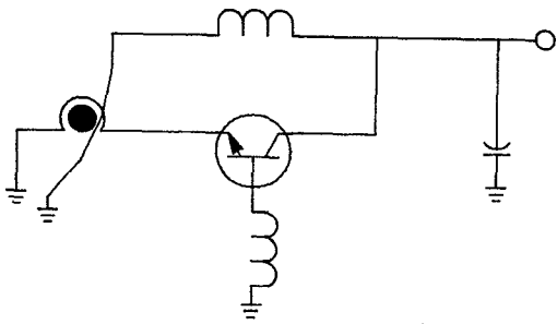
Fig.1 Composite Feedback YTO
