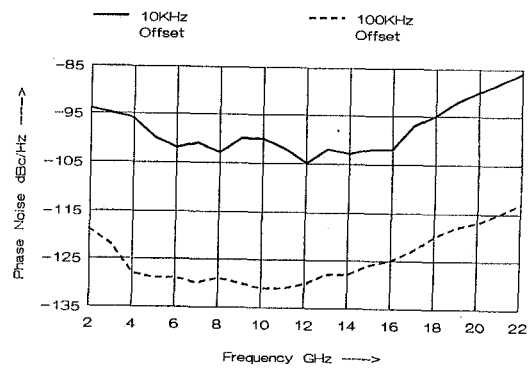
Fig.6 Phase Noise vs. Frequency
