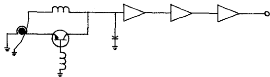
Fig.3 2-22 GHz 10 dBm YTO Block Diagram
